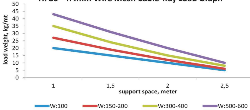
H: 35 - T:4mm Wire Mesh Cable Tray Load Graph
