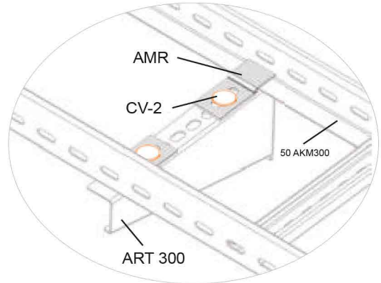
AMR BađlantýÖrneđi AMR Connection Example
