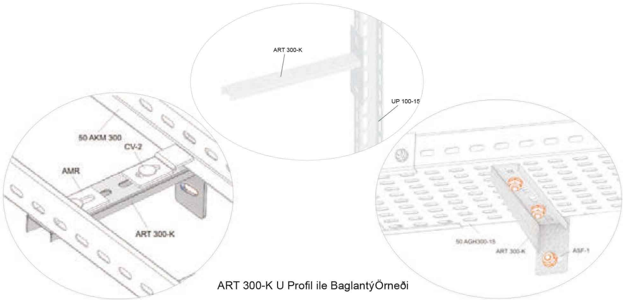
ART 300-K For U profile Connection Example
