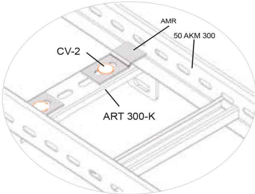
AMR BađlantýÖrneđi AMR Connection Example
