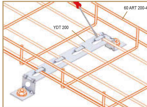
YDT Serisi Yere Montaj Örneği YDT Series to Fix Floor Example Connection View
