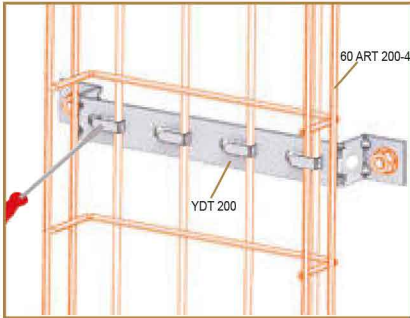
YDT Serisi Duvara Montaj Örneği YDT Series to Fix Wall Example Connection View
