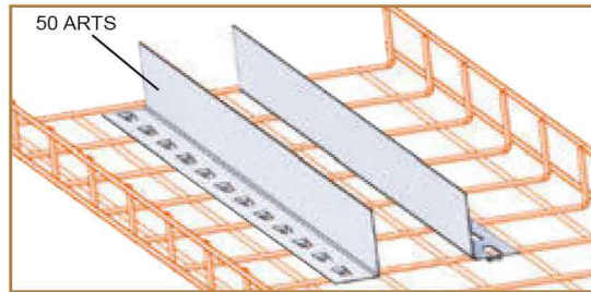
50 ARTS Connection Example
