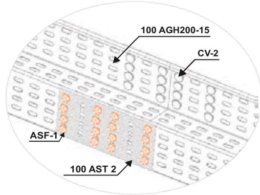
100 AST 2 Bađlantý Örneđi 100 AST 2 Connection Example
